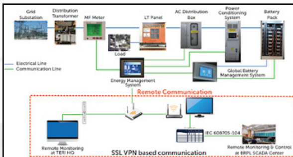
Figure 58: Schematic of Category-A Pilot by TERI/BRPL
