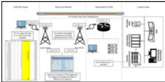
Figure 80: B&McD testbed architecture
