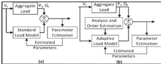
Figure 27: Measurement based (a) traditional, (b) proposed approaches for load modelling
