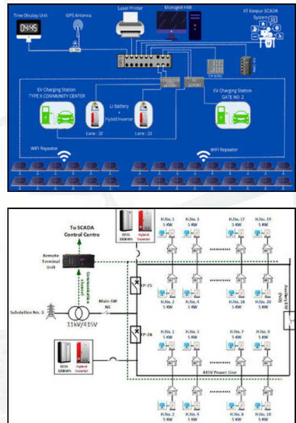
Figure 52: Communication Architecture and HMI interface
