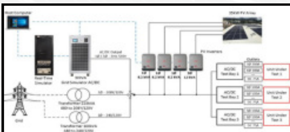
Figure 77: HIL testbed block diagram
