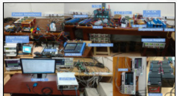
Figure 69: An integrated microgrid system with various renewable energy sources and storage units
